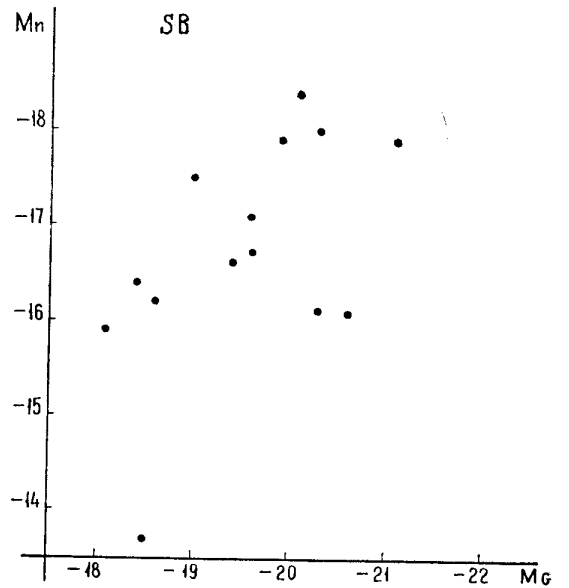
Fig. 2. The correlation between the photographic absolute magnitudes of galaxies ( M_G ) and their nuclei ( M_n ) for SB galaxies. Only the galaxies with prominences 4 and 5 are shown. The galaxies with prominence 3 would place somewhere in the lower part of the diagram, thus increasing the dispersion of points.
