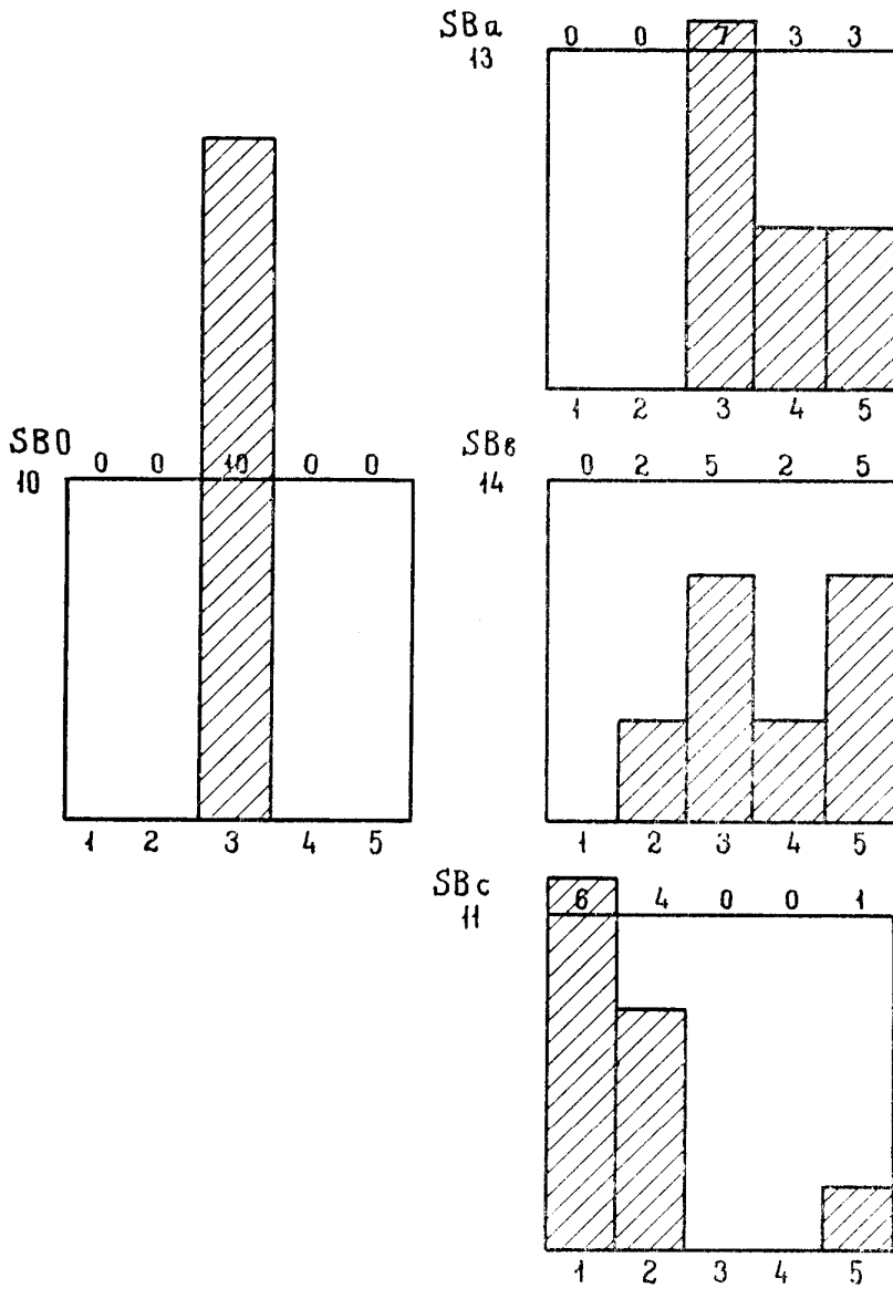
Fig. 1. Histograms showing the distribution of the estimates of the prominence of nuclei for different subtypes of barred galaxies. The numbers under each diagram are the estimates, and at the top are the numbers of corresponding galaxies. Under the letters designating the subtype the total numbers of galaxies of that subtype are given.
